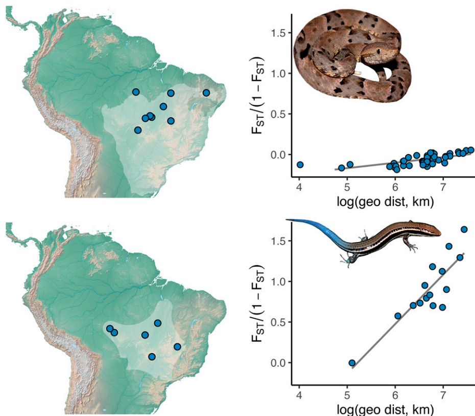
Fig. 3. Illustrative IBD slopes ( \beta_{\text{IBD}} ) generated for two species. These taxa exhibit strongly contrasting rates of population isolation: After controlling for geographic distance, the viper Bothrops moojeni ( n = 10 , Top) has a low rate of divergence between populations, whereas the gymnophthalmid lizard Micrablepharus atticolus ( n = 6 , Bottom) shows a high rate. Maps illustrate geographic ranges (see SI Appendix for information on reconstruction) for each taxon along with sampling points. Scatter plots show how genetic differentiation (as measured by F_{\text{ST}} ) accumulates across space. SI Appendix, Fig. S8 shows IBD plots across all taxa.
