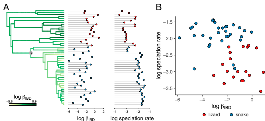
Fig. 4. Correlation between population isolation ( \beta_{\text{IBD}} ) and speciation rates ( \lambda_{\text{cladS}} ) across squamate reptiles. (A) \beta_{\text{IBD}} exhibits phylogenetic signal, as might be expected if it tracks intrinsic organismal traits such as dispersal capacity. Snakes (node “S”) are nested within squamates; all other lineages are traditionally known as “lizards.” (B) \beta_{\text{IBD}} is not significantly correlated with speciation rate (PGLS r = 0.04 , P = 0.77 ), and snakes and lizards show little overlap in the bivariate space defined by \beta_{\text{IBD}} and speciation rate.
