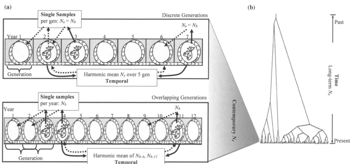
Figure 1. Time intervals over which (a) contemporary and (b) long-term N_e (effective population size) estimates apply. In (a) brackets demarcate generations and loops depict single-year breeding cycles under discrete (top) or overlapping (bottom) generations. For both single-sample estimates of inbreeding N_e and temporal methods of estimating variance N_e , solid arrows link a sample (depicted as fishes) with the parameter being estimated; dashed arrows indicate the year(s) for which the estimate pertains. Each sample is assumed to be from a single cohort before reproduction. In the discrete-generation case both single-sample and temporal methods provide an estimate of N_e per generation (gen). In (b) the time scale of long-term N_e estimates is defined by the time to the most recent common ancestor in the coalescent genealogy relating sampled gene copies.
