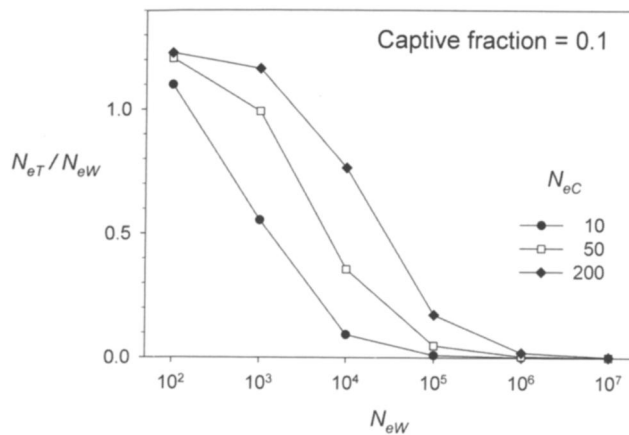
Figure 5. Effects of a single generation of supportive breeding on N_e based on Eq. 1 ( N_{eT} , total effective population size; N_{eW} , presupplementation effective population size; N_{eC} , effective population size in the hatchery; captive fraction, proportion of individuals successfully reproducing in the wild that were produced in the hatchery).
