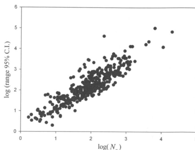
Figure 3. Precision as a function of the magnitude of empirical point estimates for contemporary N_e (effective population size) (Palstra & Ruzzante 2008). Only estimates with finite upper confidence limits are included, so the observed relation is biased toward better precision at higher N_e .
