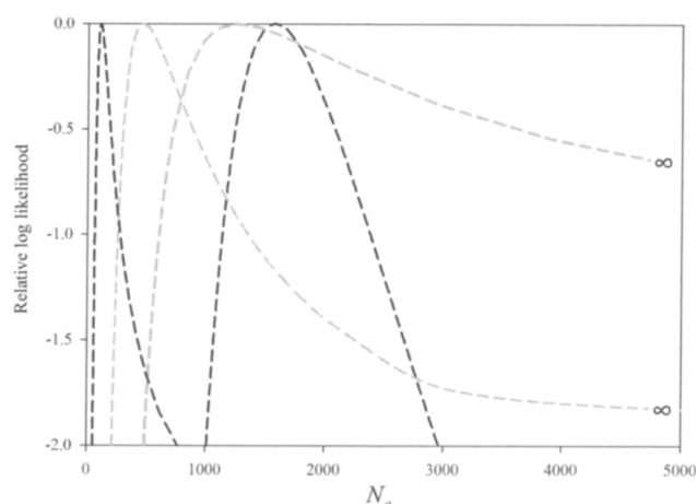
Figure 4. Pseudo-maximum likelihood profiles of variance N_e (effective population size) estimates calculated using the method of Wang (2001) with temporal genetic data (13 microsatellites) for Atlantic salmon from four rivers (F. Palstra, unpublished data). In these examples, a relative log-likelihood value of zero corresponds to the point estimate of N_e and a value of -2 corresponds to the outer limits of the 95% CIs (black, two estimates with finite confidence limits; grey, two estimates with infinite upper confidence limits).
