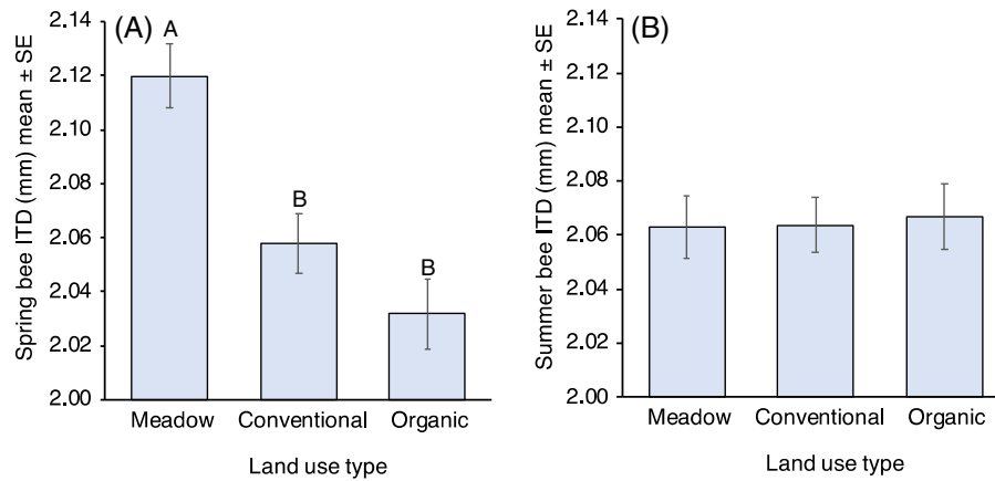
FIGURE 2 Body size of Agapostemon virescens female bees at three land use types including unmowed meadows, conventional pesticide application and mowed agricultural and organic pesticide free mowed landscapes. Inter-tegular distance (ITD) (mm) mean \pm standard error (SE) for (a) spring bees and (b) summer bees is shown. Uppercase letters indicate statistical significance. Y-axis scales from 2.0
