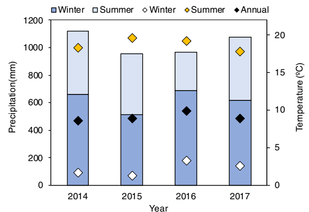
FIGURE 3 Climate data for Durham (NH, USA) for the years 2014–2017. Yearly amount of precipitation is shown as stacked bars, winter (dark blue) and summer (light blue), and mean temperature (°C) as diamonds, annual (black), winter (white) and summer (yellow) for each year
