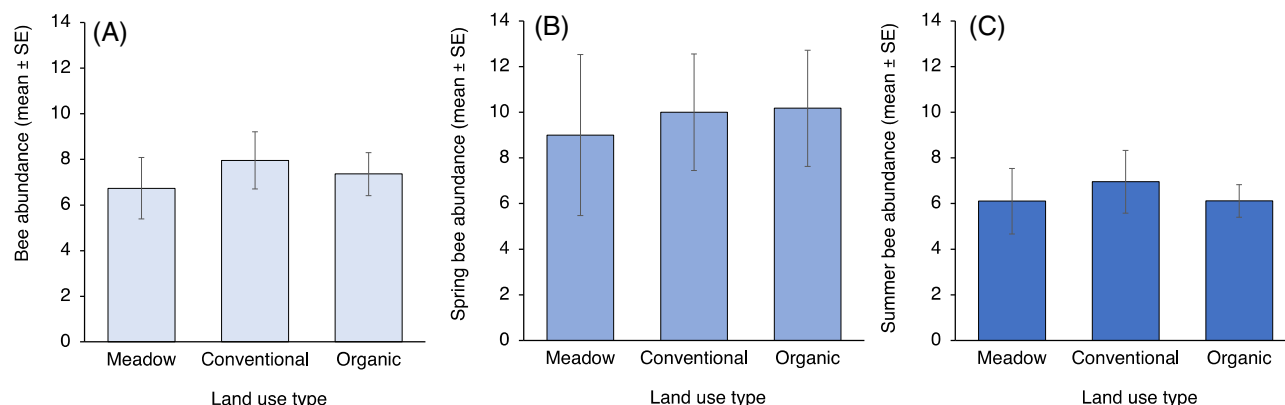
FIGURE 1 Abundance of Agapostemon virescens female bees at three land use types collected throughout three consecutive years (2015–2017), showing (mean ± SE per transect) for (a) overall bee, (b) spring and (c) summer bee abundance
